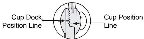
Figure 2-13 Cup Docking Interlock
