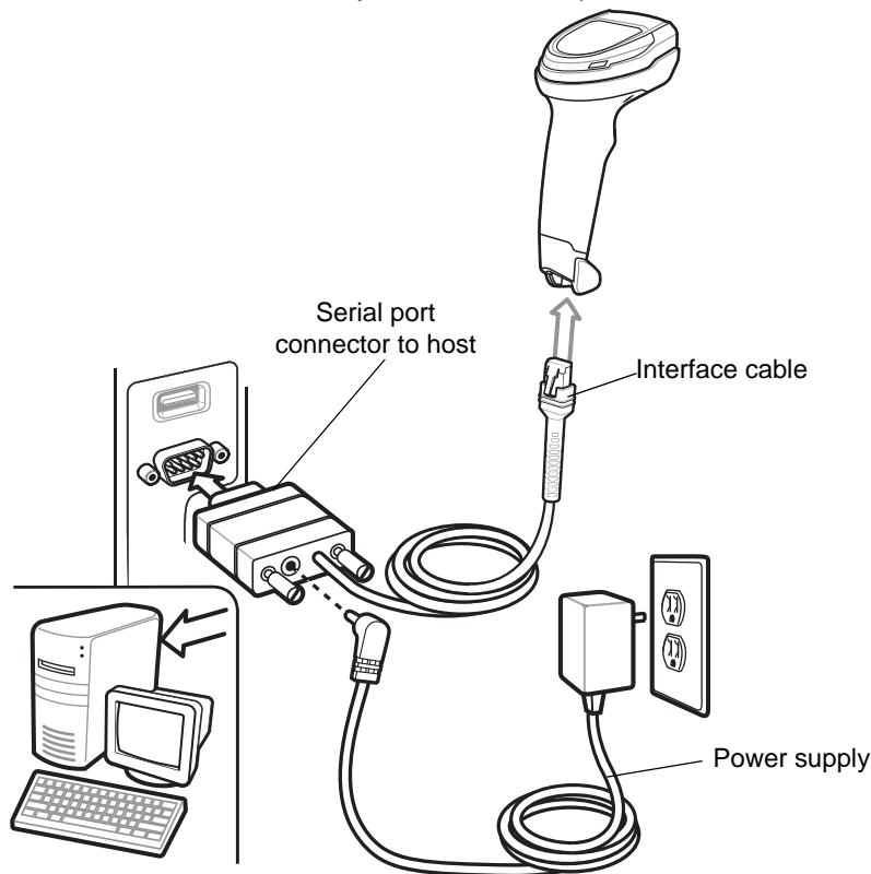
Figure 6-1 RS-232 Connection
