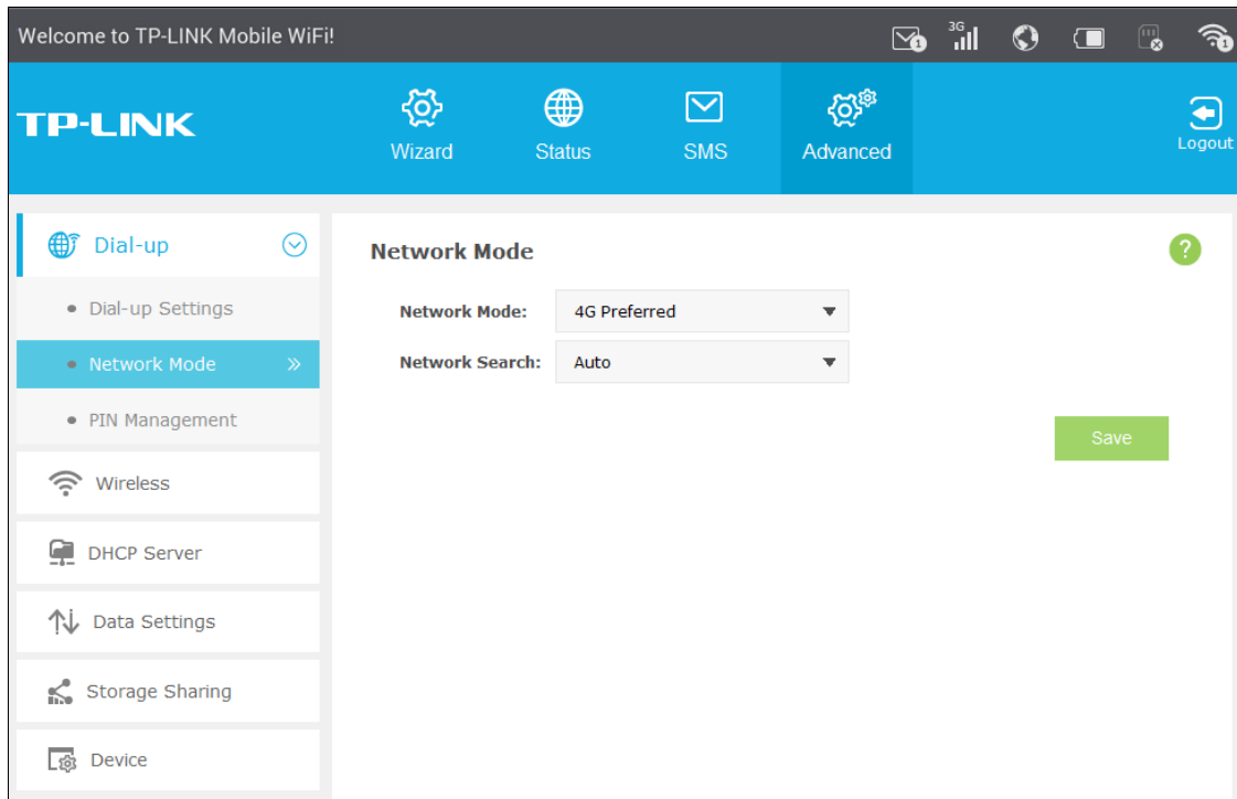
Figure 4-14 Network Mode Settings
