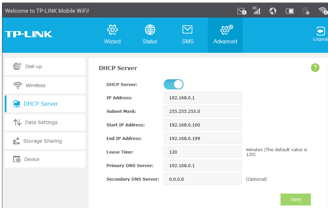
Figure 4-22 DHCP Server
