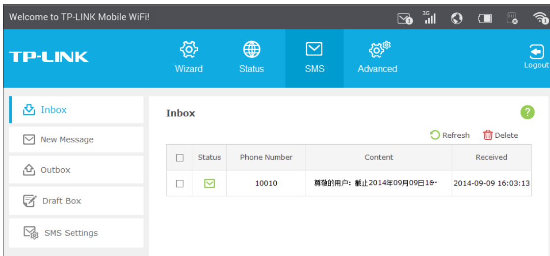
Figure 4-4 Inbox
