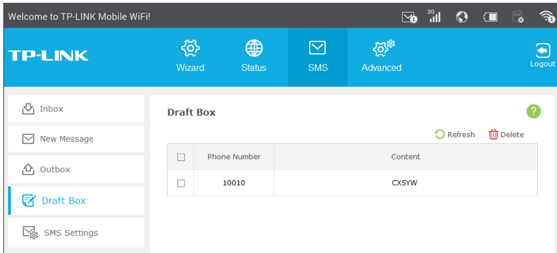
Figure 4-7 Drafts Box
