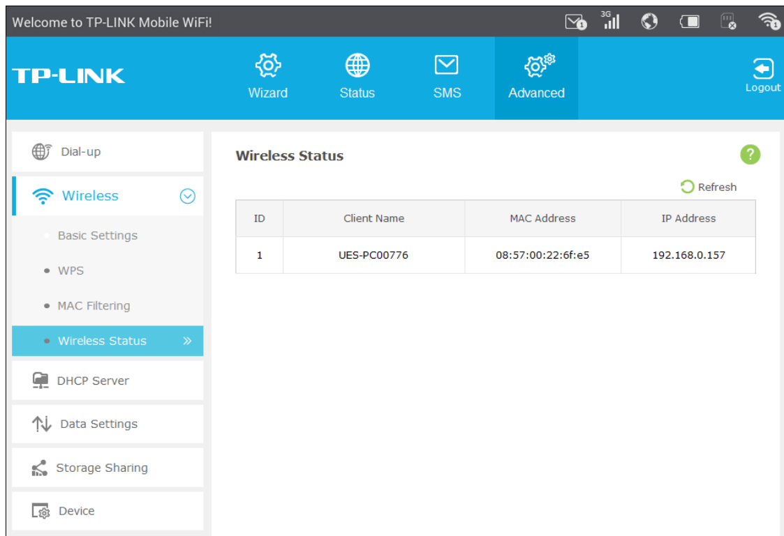
Figure 4-21 Wireless Status
