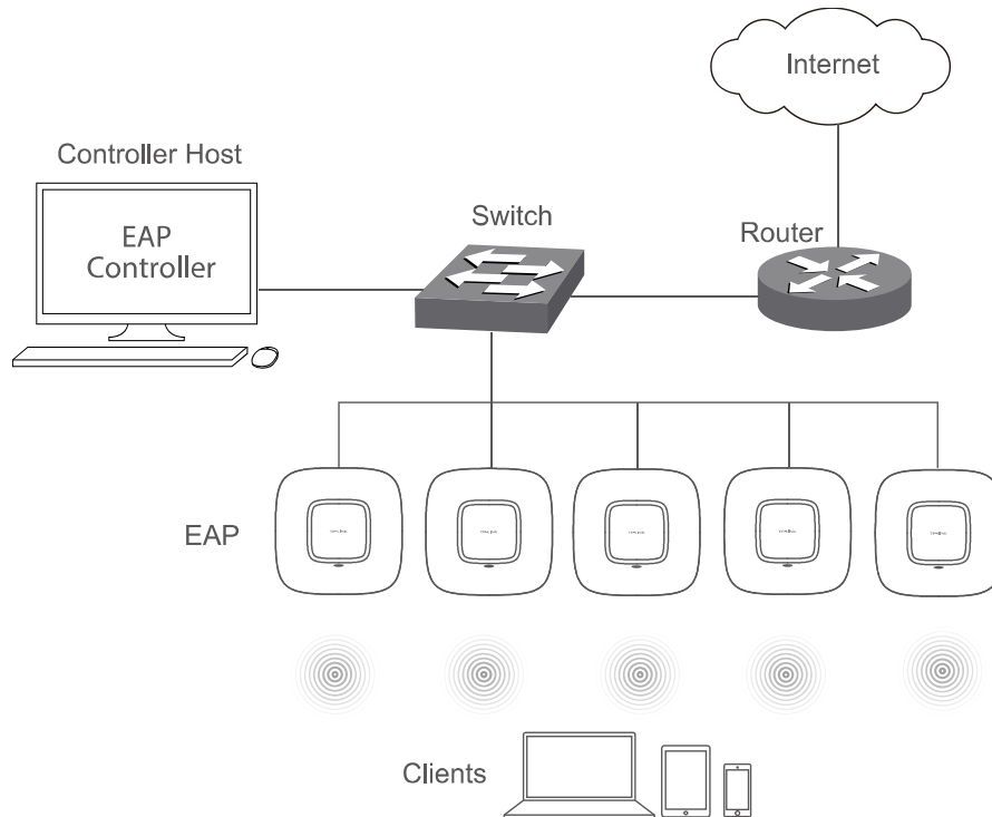
Figure 2-1 Typical Topology
