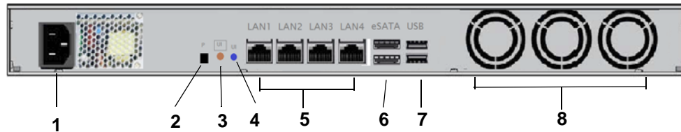
Figure 11. Rear panel
