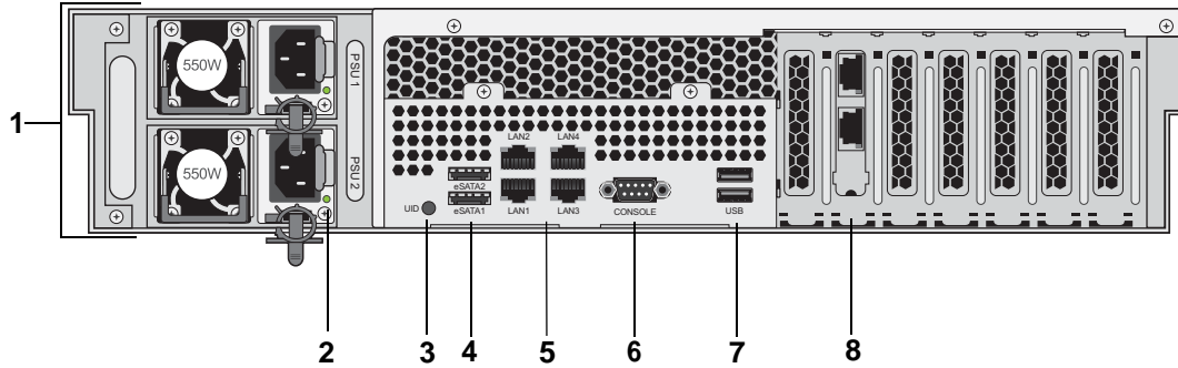
Figure 16. Rear panel
