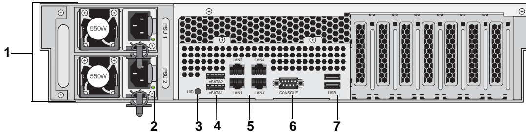
Figure 15. Rear panel
