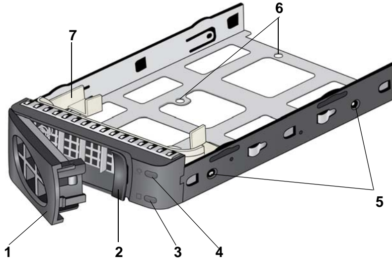
Figure 17. Disk tray
