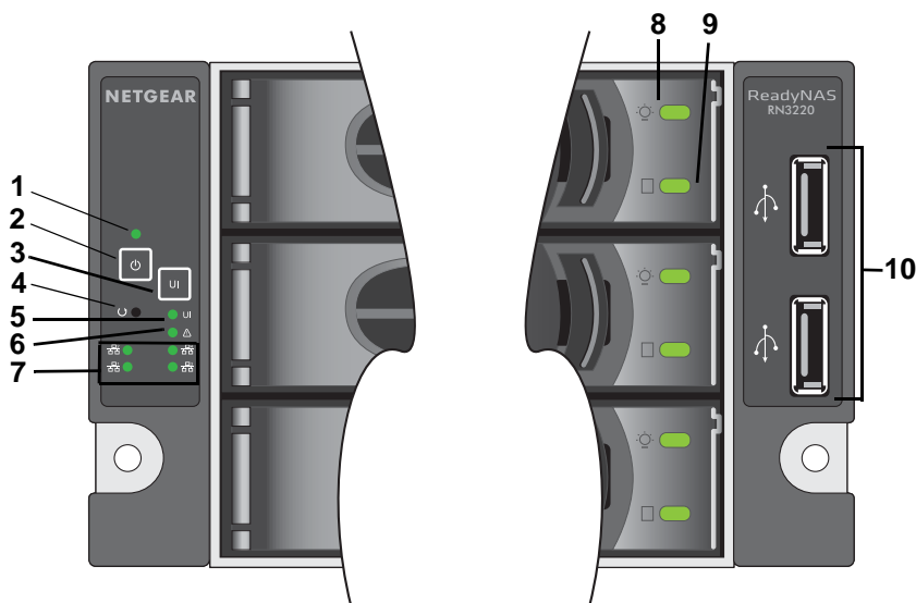
Figure 13. Control panel
